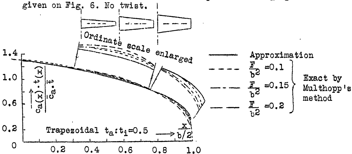
Figure 6.- Comparison curves for t_a:t_i=0.5 for various values of F/b^2 . No twist.
