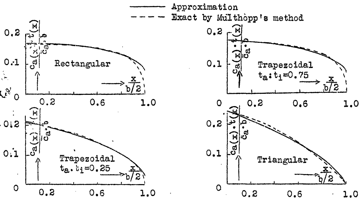
Figures 2 to 5.- Comparison curves with b^2/F=6.67 for various taper ratios. The comparison for t_a:t_i=0.5 is given on Fig. 6. No twist.
