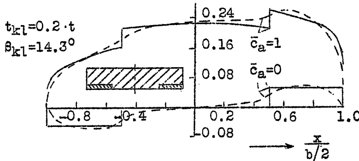
Figure 12.- Comparison curves for a rectangular wing with b^2/F=5 for an aileron deflection \beta=0.25 \approx 14^\circ with and without lift. The corners of the approximation curve can practically be well rounded off by hand following the example given and thus considerably better agreement is obtained. The rolling moments of the non-rounded off approximation curve very well agree with the exactly computed values.
